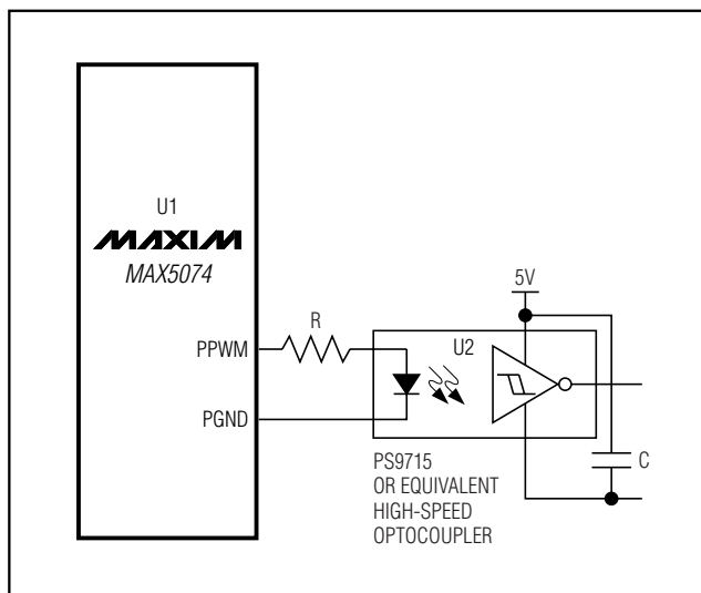
Figure 2. Secondary-Side Synchronous Rectifier Driver Using a High-Speed Optocoupler
