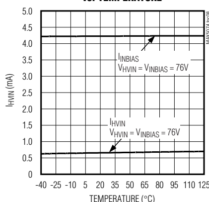
HVIN AND INBIAS INPUT CURRENT vs. TEMPERATURE
