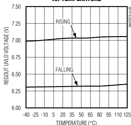
REGOUT UVLO VOLTAGE vs. TEMPERATURE
